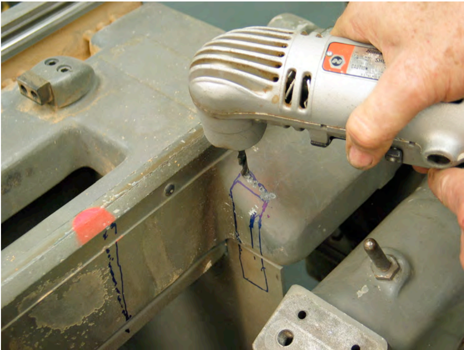
Figure 245 Drill a line of holes that are very close together.
