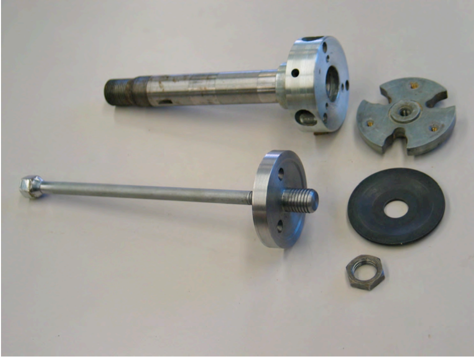
Figure 26 This is the new threaded faceplate showing the Unisaw nut and the Unisaw blade flange. Using the original arbor limits blade height above the table.
