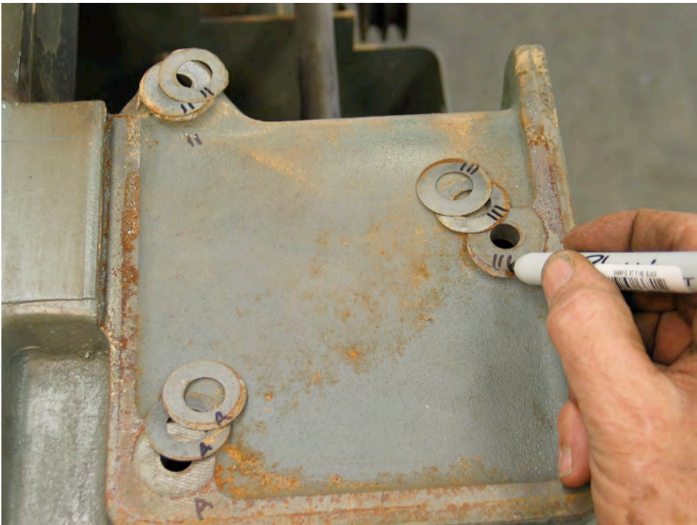
Figure 19 Mark well where the factory shims go.
