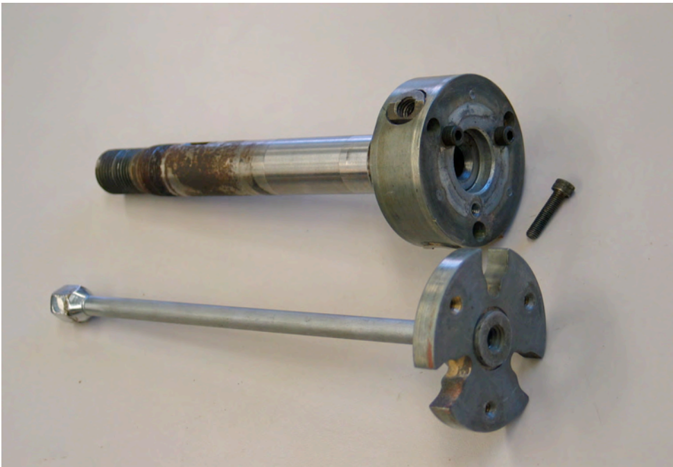
Figure 25 This is the original faceplate with drawbar and original shaft. The faceplate method uses the original shaft so a new one doesn't have to be made. The new faceplate will fit into the recess and be held in by the drawbar and the three perimeter 10-32 socket head cap screws.
