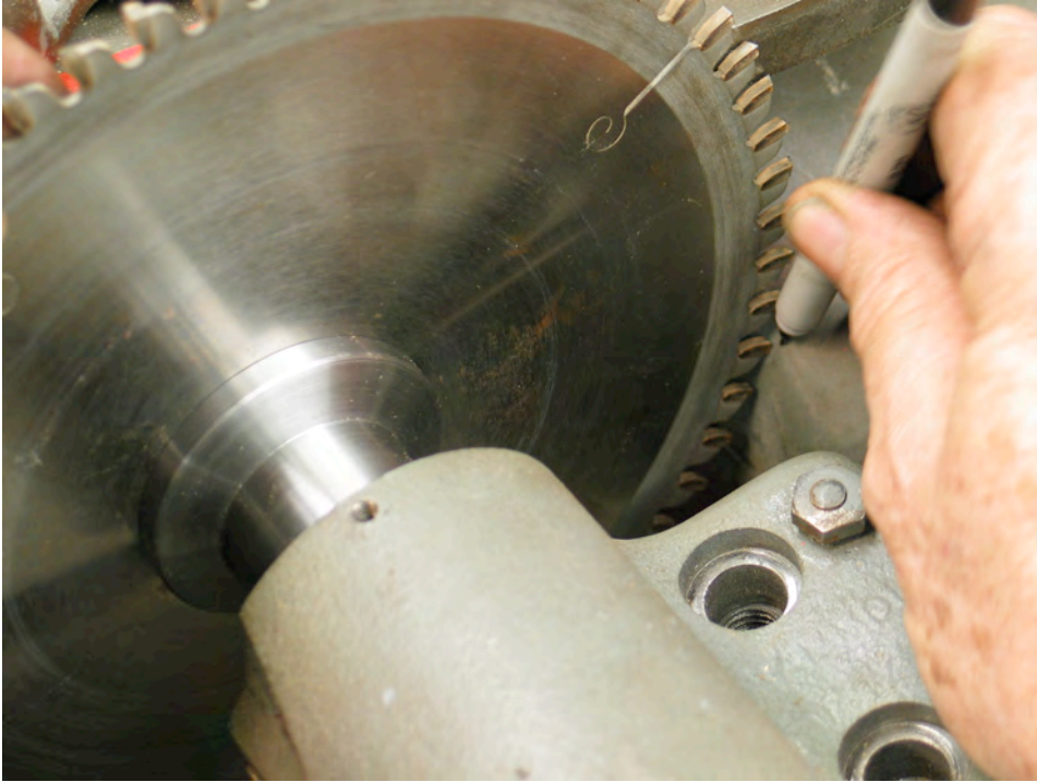
Figure 3222 With the 8-1/5" blade in the upper position, observe where the cuts need to be made and mark plenty of clearance with a marker. Keep in mind that the blade has to move laterally to come off the shaft.
