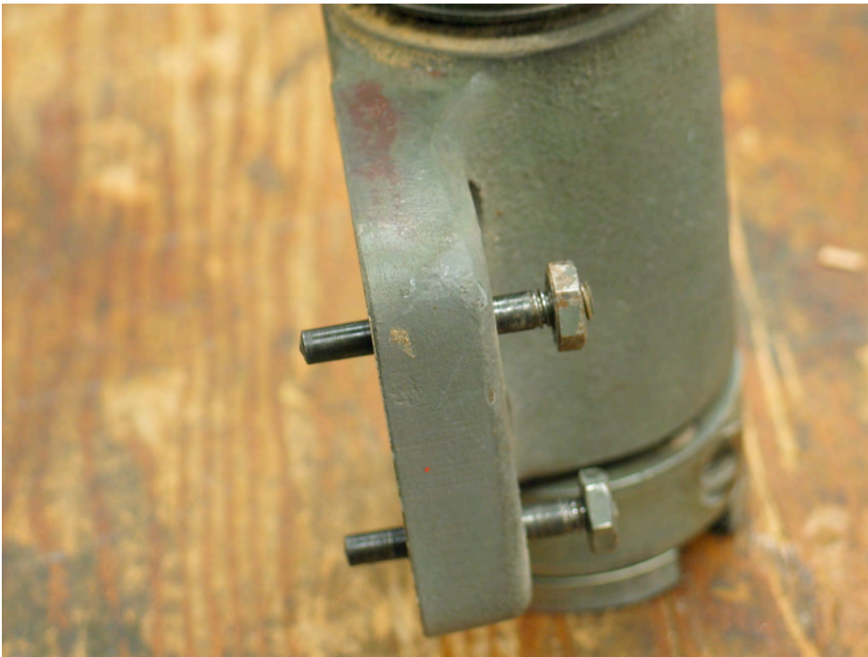
Figure 5 A detail of the threaded top locating pins with nuts.
