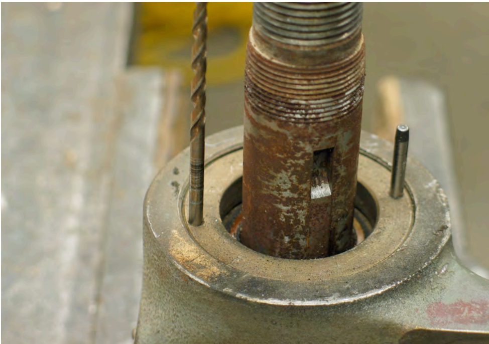
Figure 13 Under the pulley is another spanner ring holding the position of the outer race of the bearing. There is one of these rings on each side of the arbor housing. The arbor will have to be pressed out, putting pressure on the pulley end (shown here)
