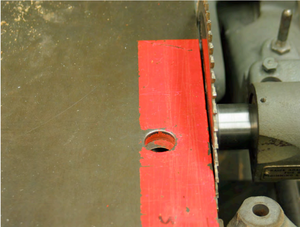
Figure 324 A 1/16" clearance will do nicely.
